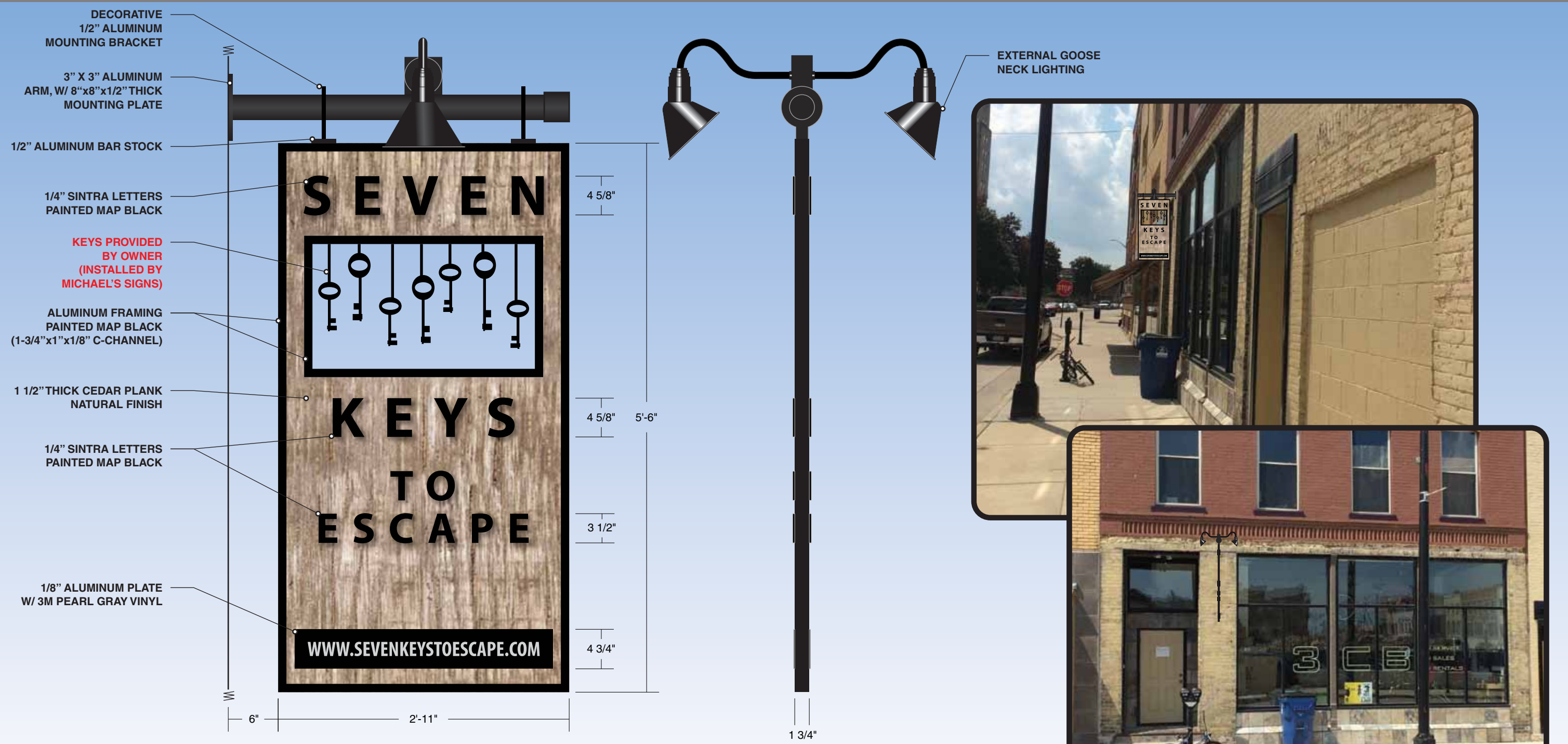
SEVEN KEYS TO ESCAPE / BUILDING SIGN ONE (1) DOUBLE SIDED, EXTERNALLY ILLUMINATED FLAG MOUNTED SIGN 1 3/4" DEEP ALUMINUM FRAME (MAP BLACK) W/ CEDAR PLANK SIGN BODY ROUTED 1/4" SINTRA LETTERING PAINTED MAP BLACK SEE SPEC. ABOVE
