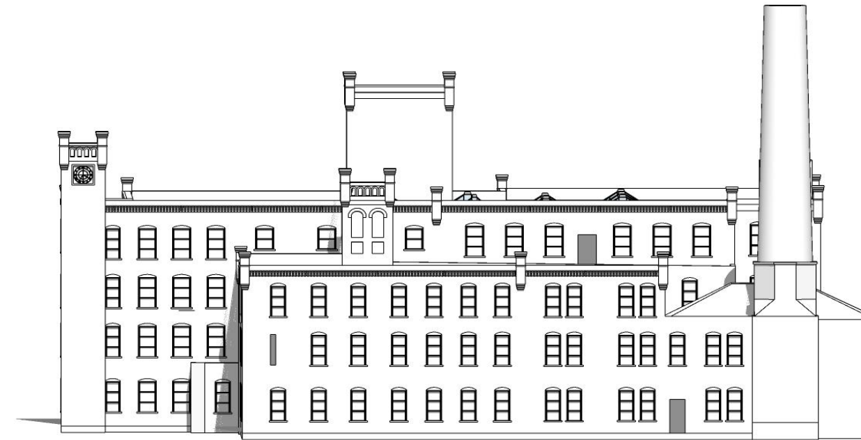
2200 SOUTHEAST ELEVATION
