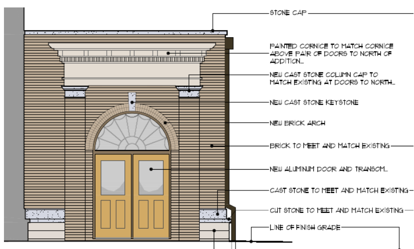
Proposed Building Addition Rendering (east side), submitted by applicant
