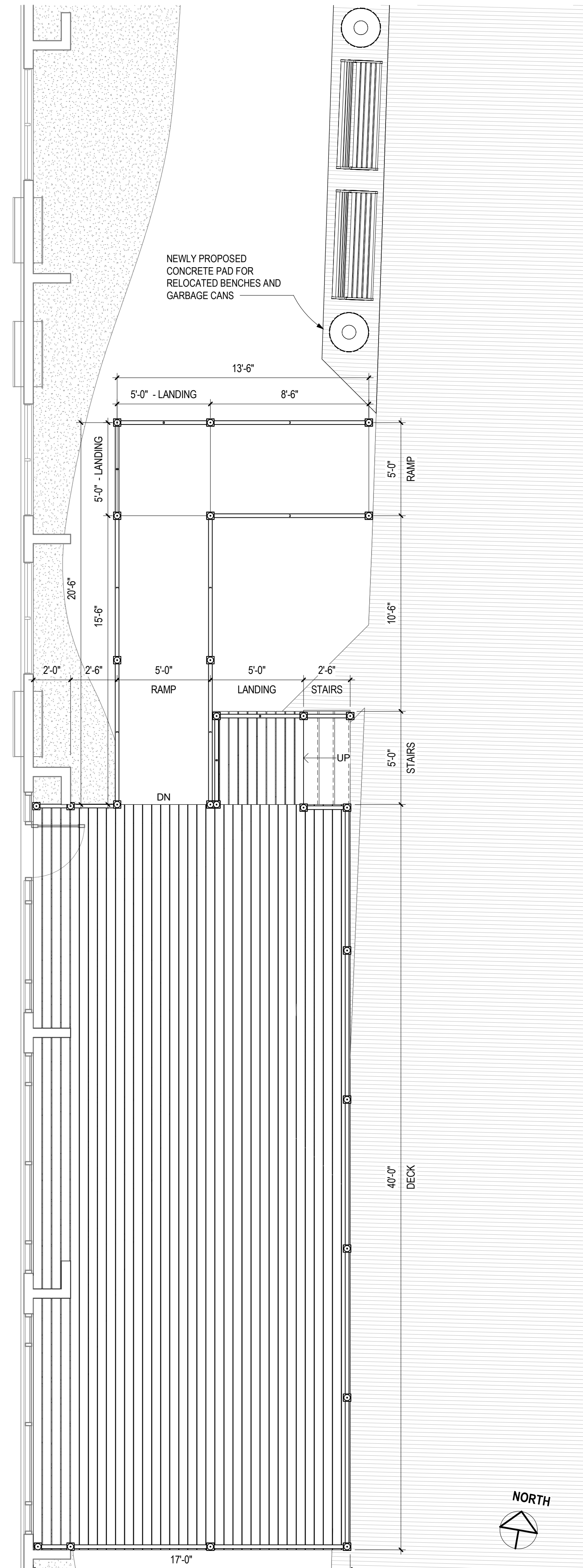
AREA PLAN WITH PROPOSED DECK
